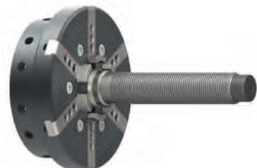
QuickHub open, max. clamping range 77,1 mm (with additional attachments).
